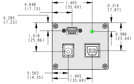
Back Panel USB 2.0
